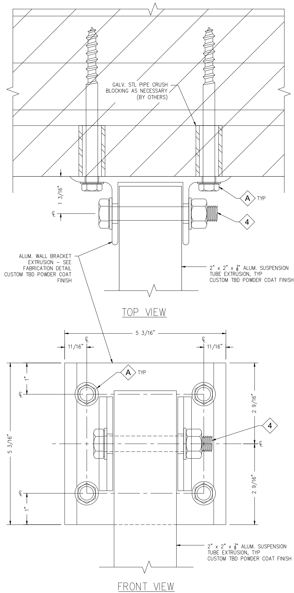
1 4 CANOPY WALL PLATE DETAIL SECTION/ELEVATION N.T.S.
