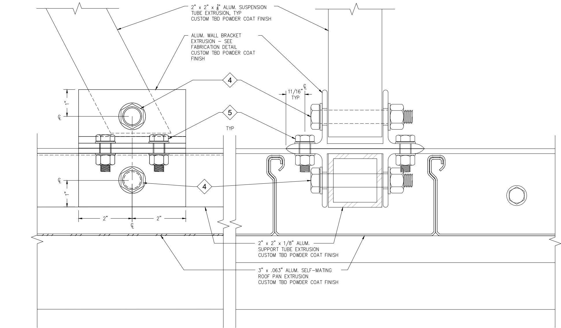
2 4 CANOPY SUSPENSION ATTACHMENT DETAIL SECTION/ELEVATION N.T.S.
